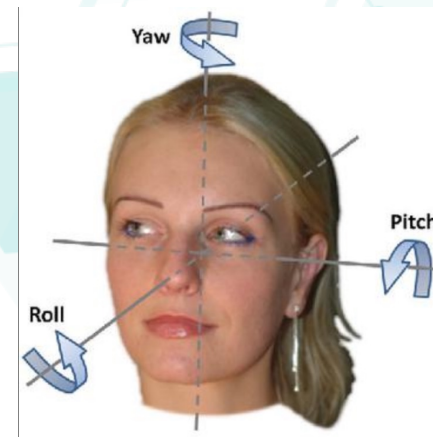
Pose Estimation
