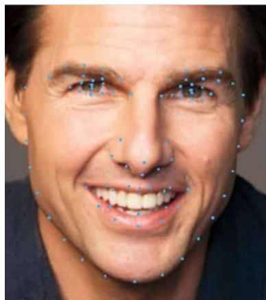
Landmark detection
