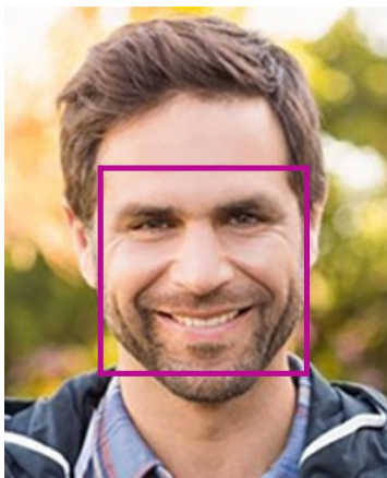
Face detection
